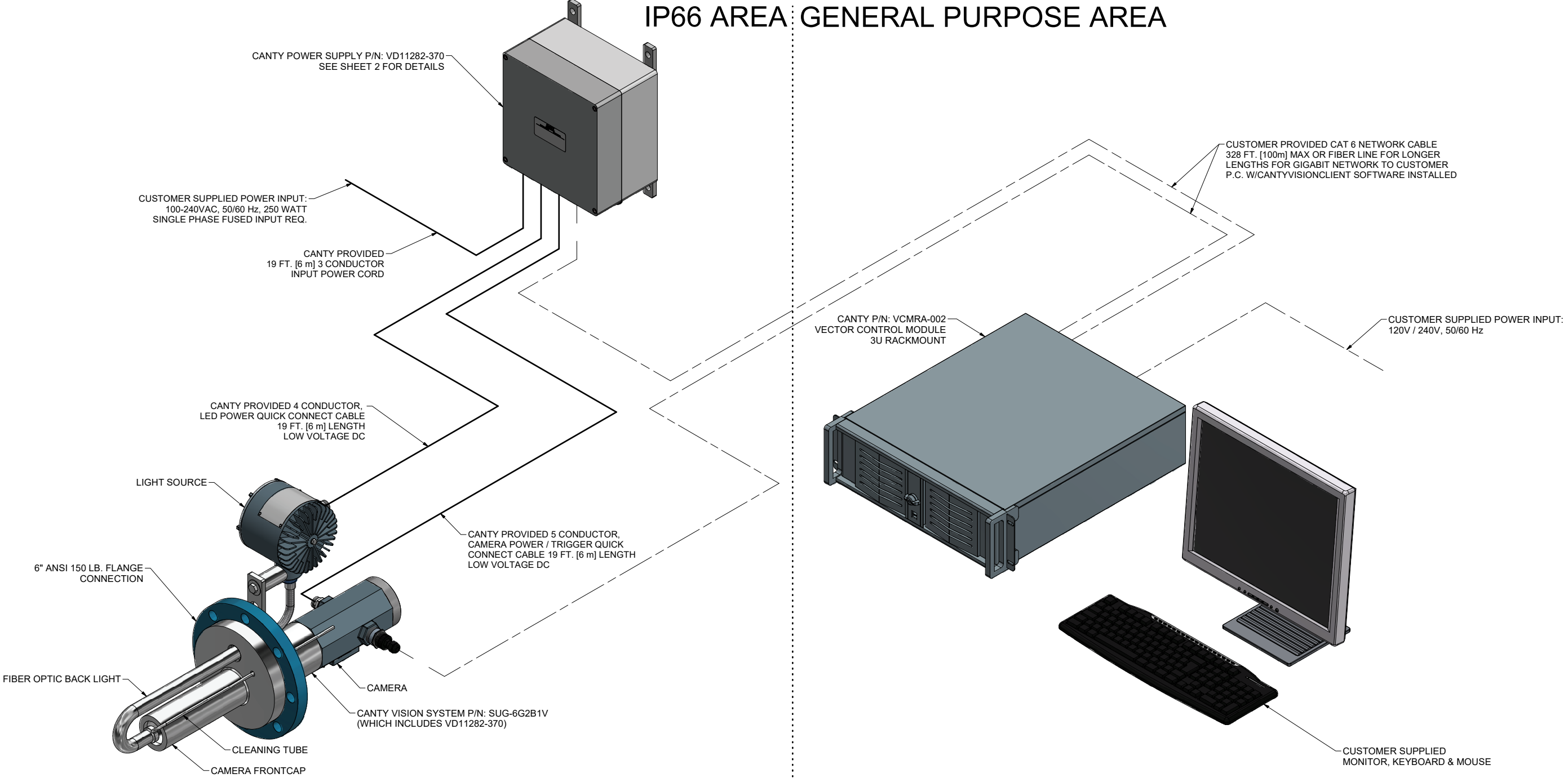
ISOMETRIC VIEW SCALE .25 : 1
