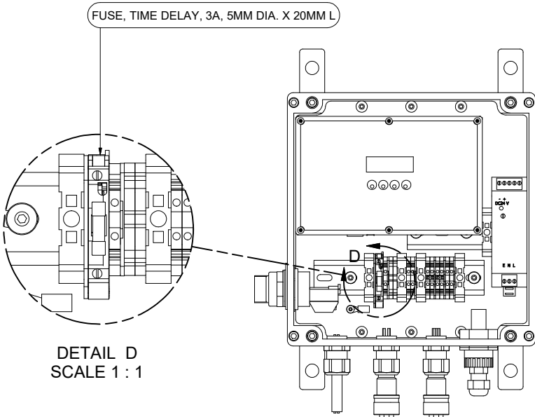
FRONT VIEW SCALE .375 : 1 (COVER REMOVED)
