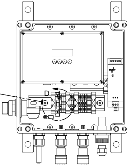
FRONT VIEW SCALE .375 : 1 (COVER REMOVED)
