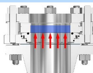
Seal Under Positive Pressure
