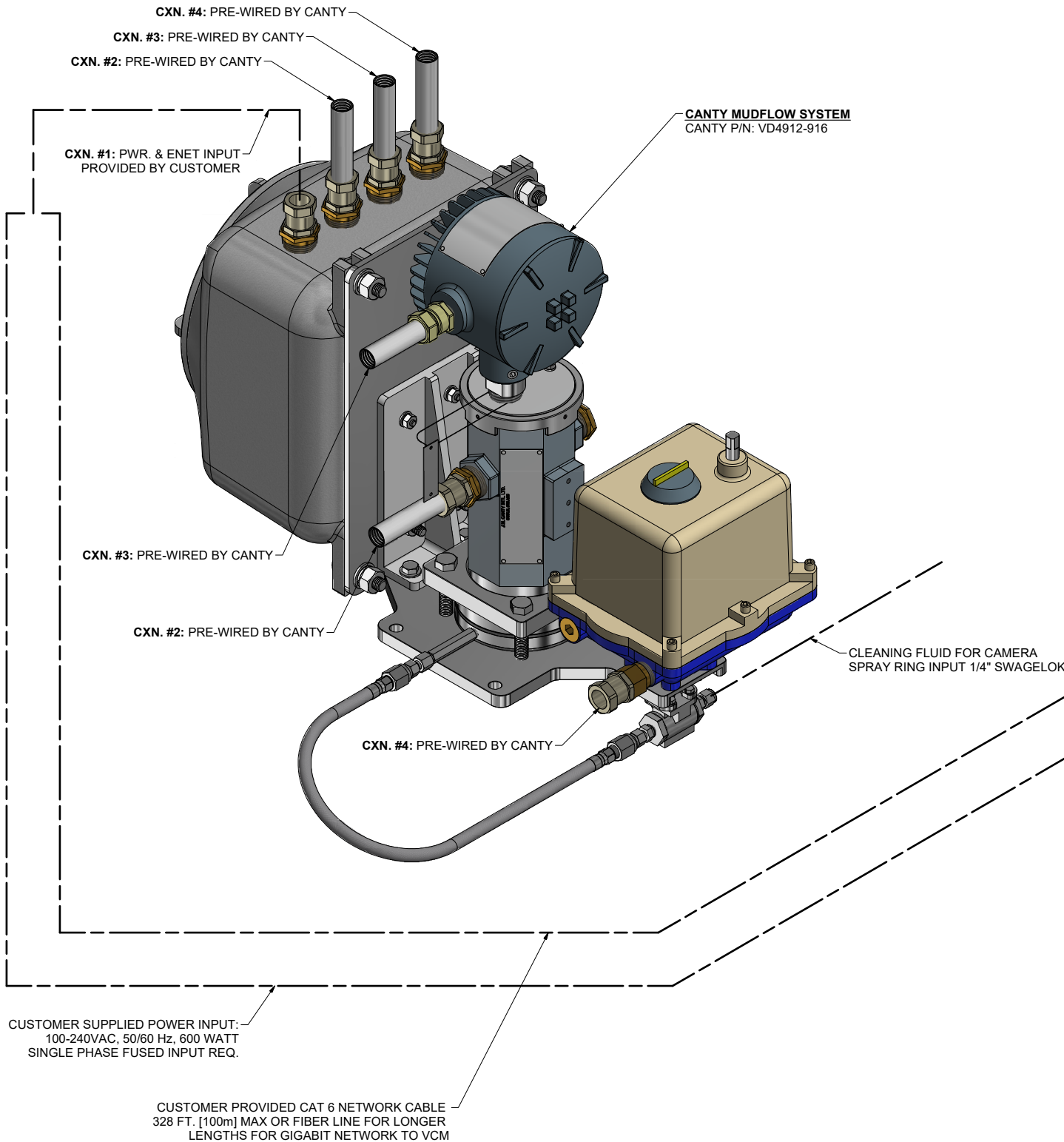
ISOMETRIC VIEW SCALE .375 : 1
