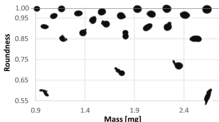
Figure 3. Shape and mass relationship of S230 shot. Images of individual S230 shot particles taken using the JM Canty SolidSizer. Particle mass, M = \rho(\pi/6)D_{eq}^3 , where the density of steel, \rho = 7.8 \text{ g/cm}^3 .
