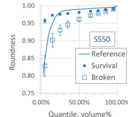
Figure 4: Plot characterizing shot after 1500 cycles in the Ervin Tester. The reference line represents the shape of the as-received shot from Ervin. The solid points represent the shot that remained unbroken and lies to the right of the threshold line on Figure 4. The open points represent the broken shot to the left of the threshold line.
