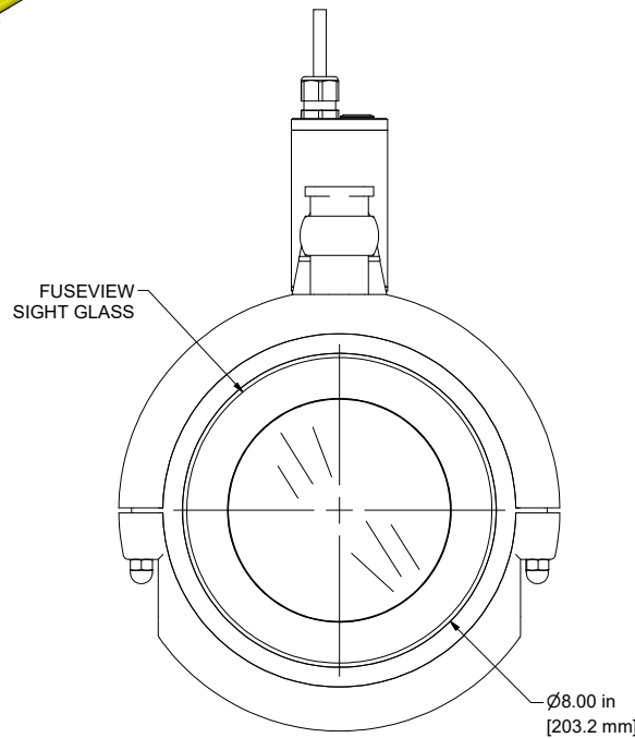
BOTTOM VIEW SCALE .375 : 1
