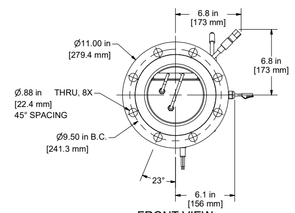
FRONT VIEW SCALE .20 : 1
