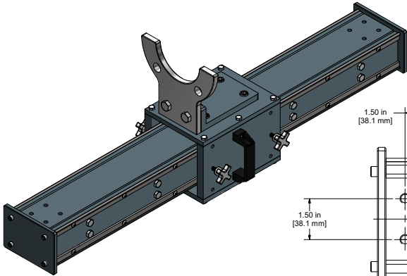
ISOMETRIC VIEW SCALE .3125 : 1
