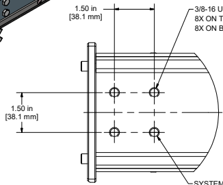
DETAIL A SCALE .625 : 1
