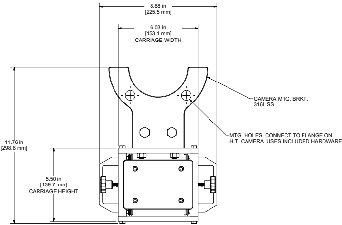
FRONT VIEW SCALE .4375 : 1
