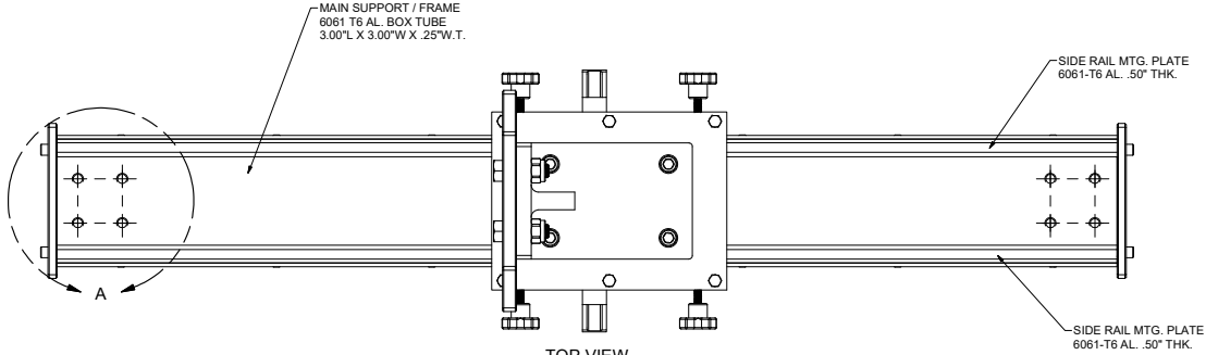
TOP VIEW SCALE .4375 : 1
